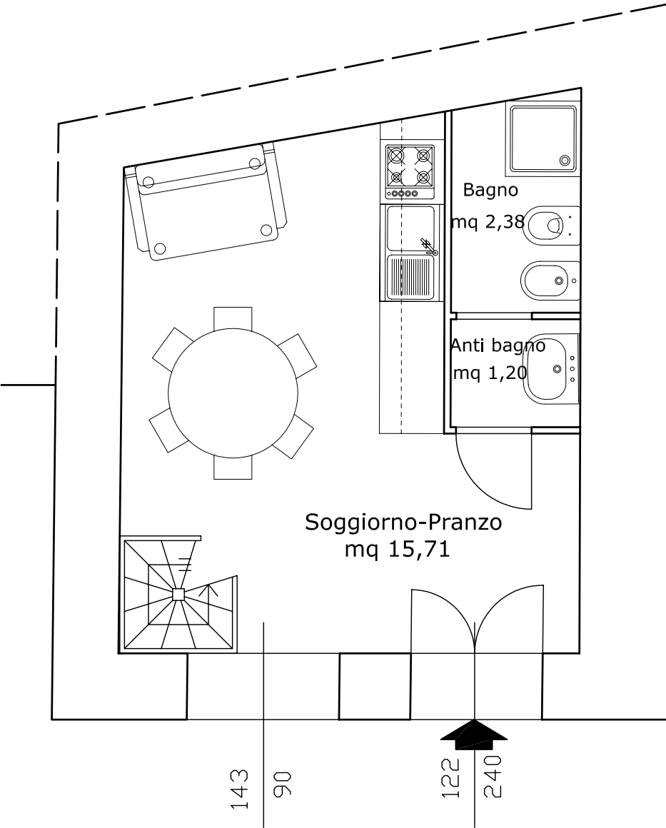
Piano terra
